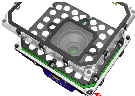
Fig. 5 - Aligning the cover (36 LEDs model)
