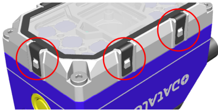
Fig. 2 - Do not force the clip locks open
