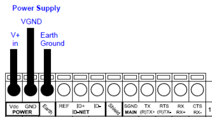
Figure 5 - Power Supply Connections
