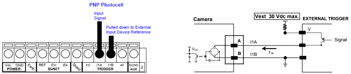
Figure 9 - PNP External Trigger Using External Power
